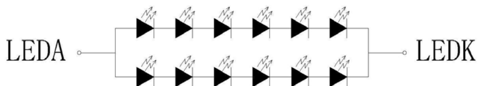
BL CIRCUIT DIAGRAM
